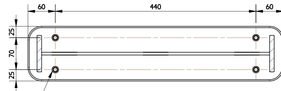
FOOTPRINT SECTION A-A SCALE 1:5
