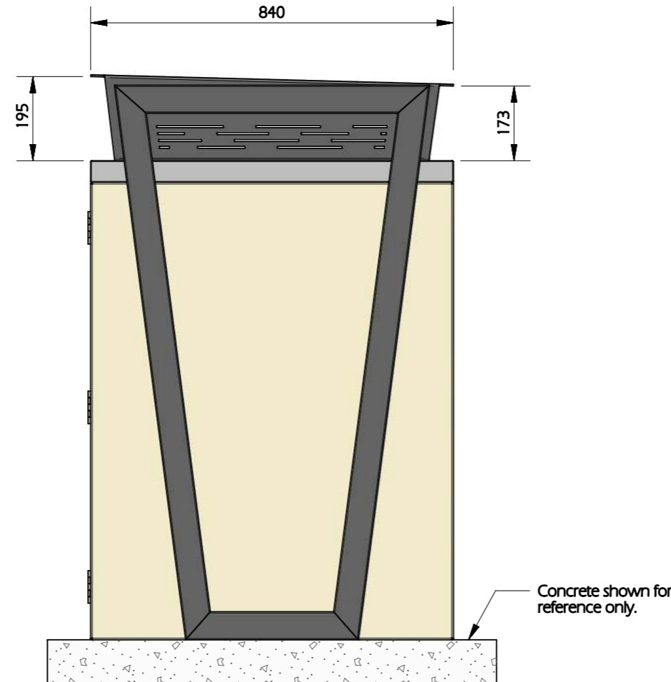
SIDE VIEW SCALE: NTS
