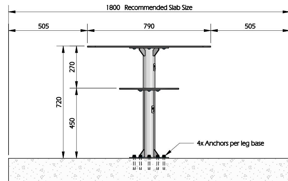
SIDE VIEW
