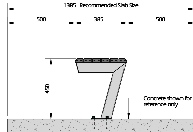
SIDE VIEW
