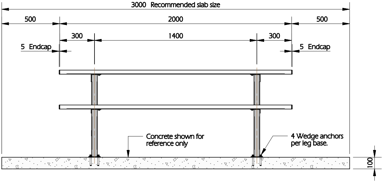
ELEVATION SCALE 1:20
