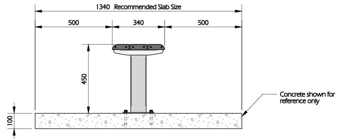
SIDE VIEW
