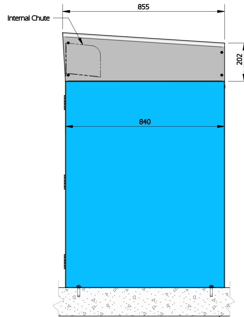
SIDE VIEW SCALE: NTS
