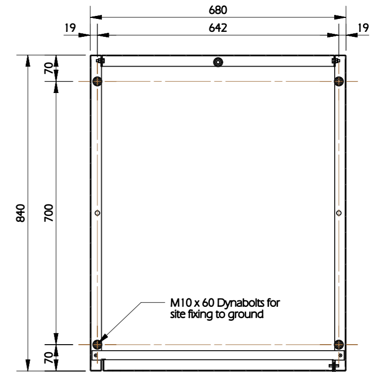
FOOTPRINT SECTION A-A SCALE 1:10
