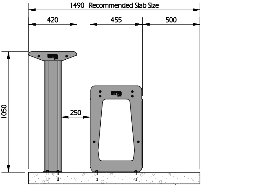
SIDE VIEW SCALE 1:20
