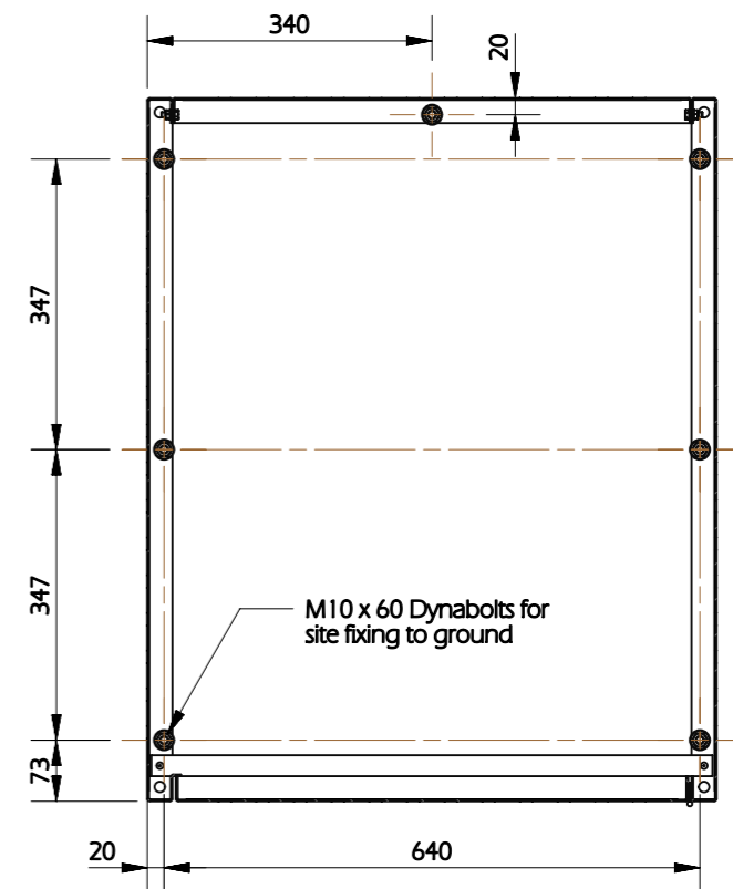
FOOTPRINT SECTION A-A SCALE 1:10
