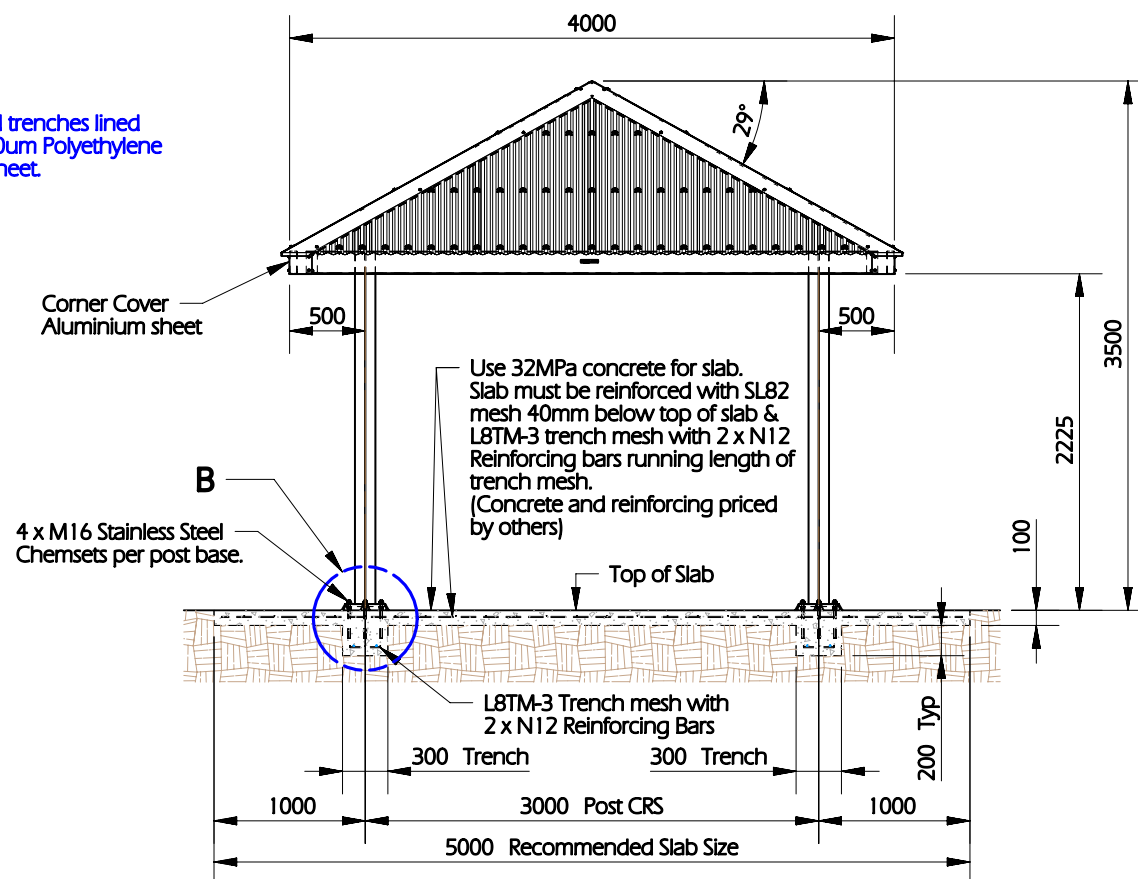
ELEVATION SCALE 1:50
