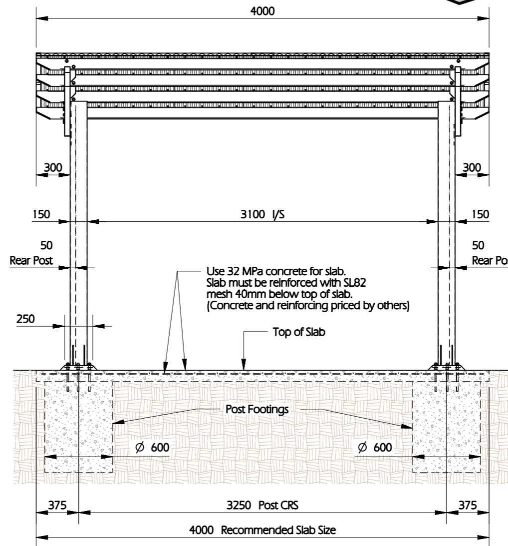
FRONT VIEW SCALE: NTS
