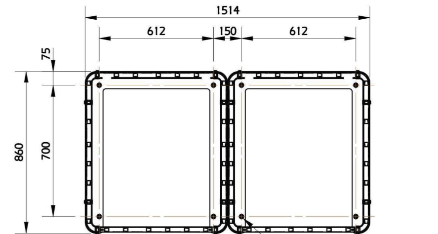
FOOTPRINT SECTION A-A SCALE 1:20
