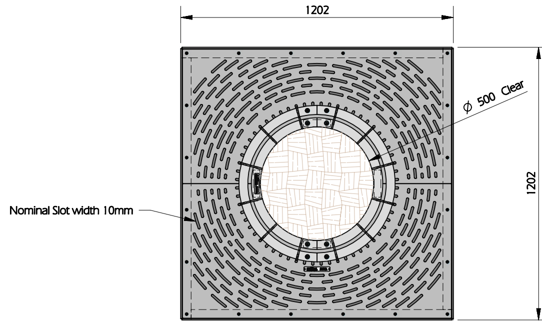
TOP VIEW
