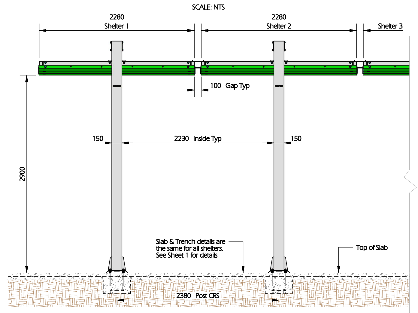
SIDE VIEW - MULTIPLE SHELTER INSTALL
