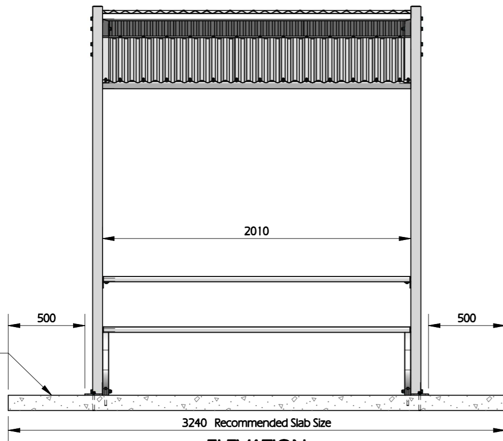
ELEVATION SCALE 1:25
