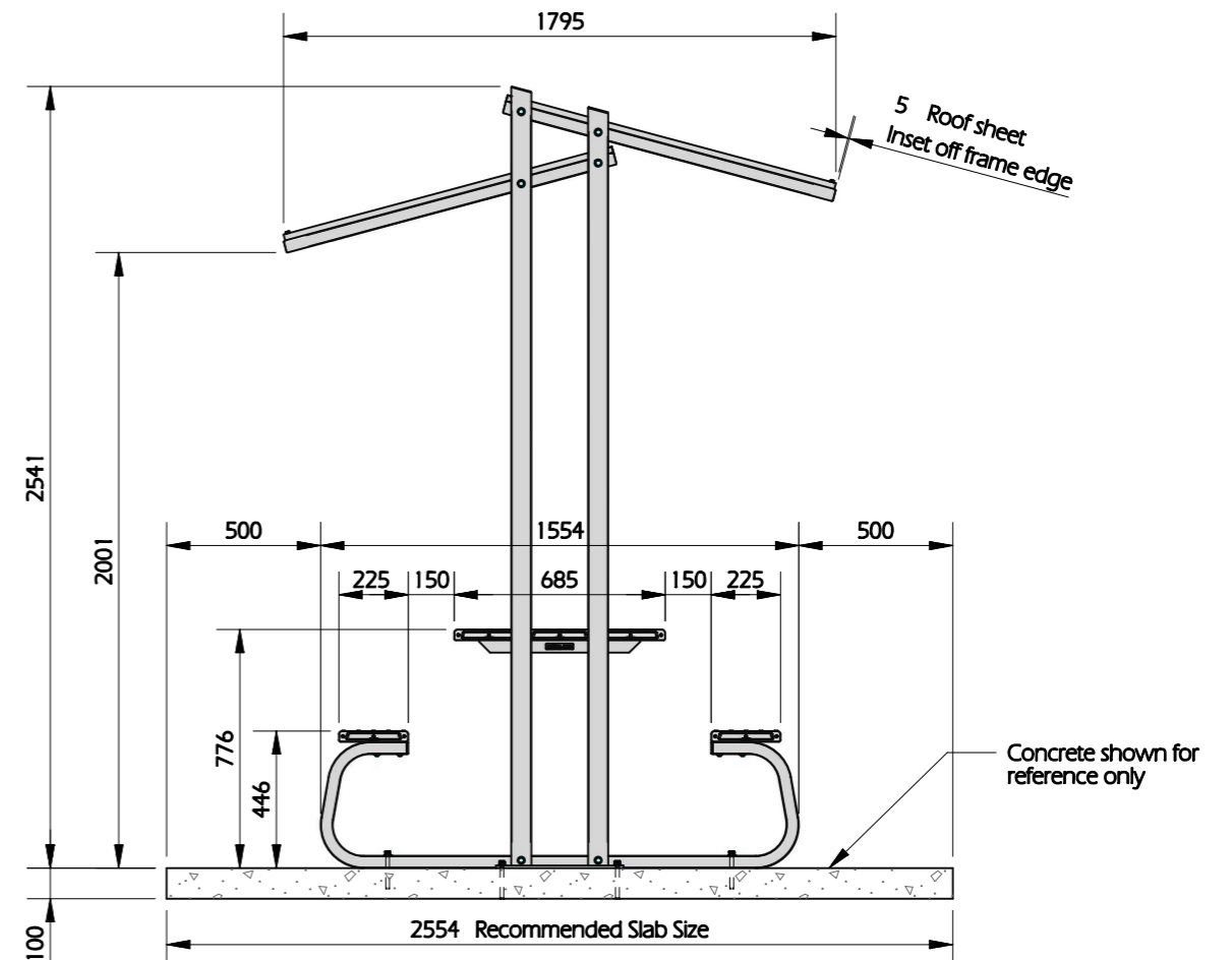
SIDE VIEW SCALE 1:25
