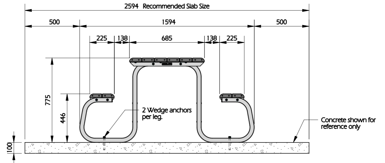
SIDE VIEW SCALE 1:20
