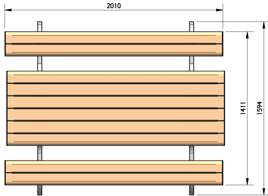
TOP VIEW SCALE 1:20
