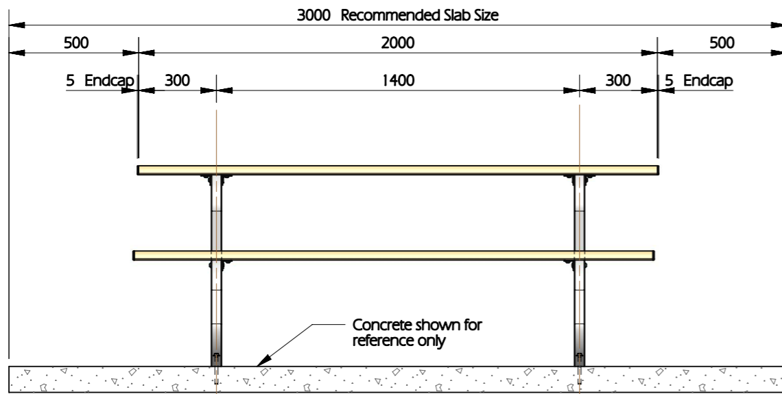
ELEVATION SCALE 1:20
