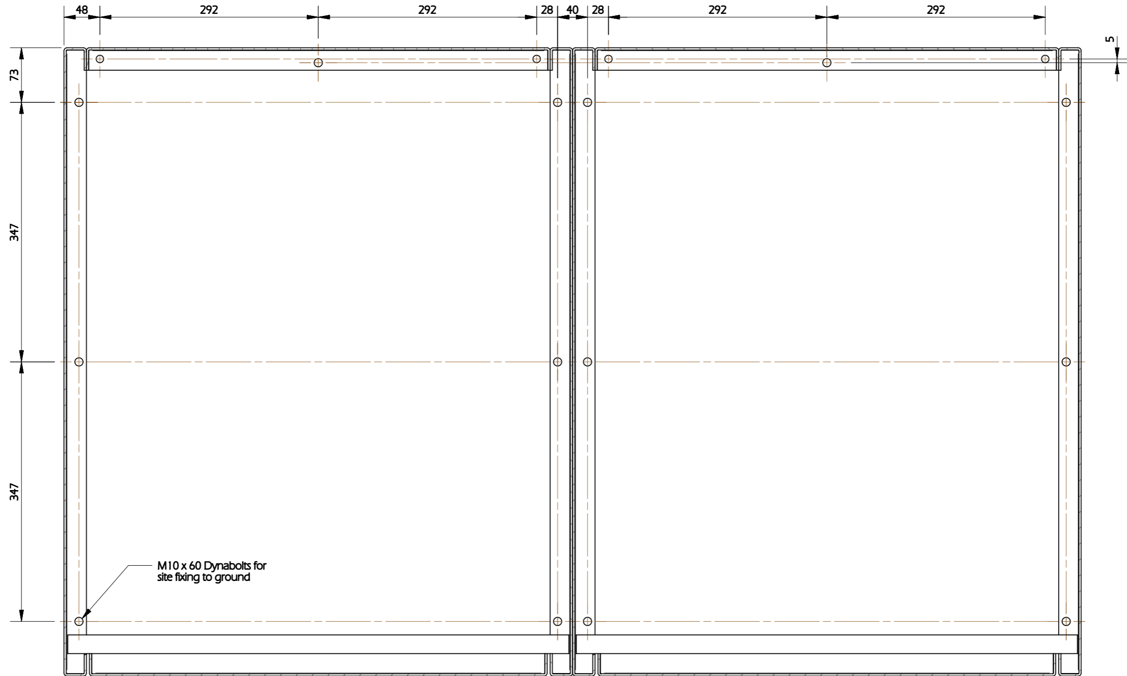
FOOTPRINT SECTION A-A SCALE 1:5
