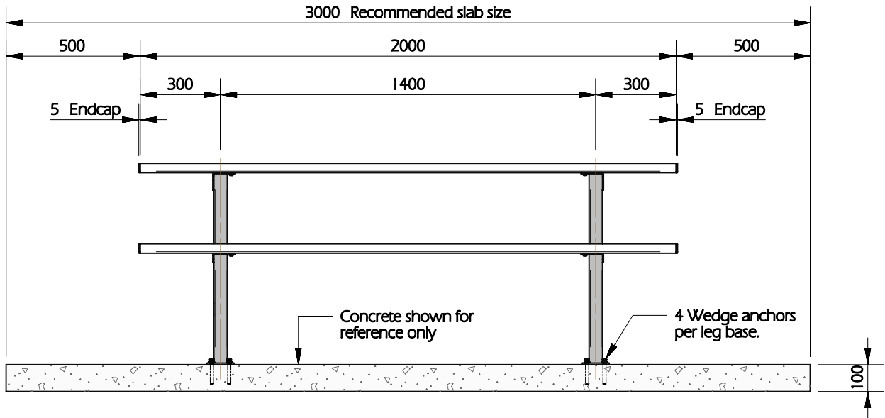
ELEVATION SCALE 1:20
