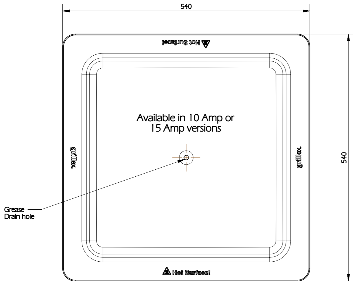
TOP VIEW SCALE 1:5
