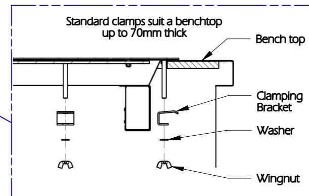
BENCH TOP CLAMPS
