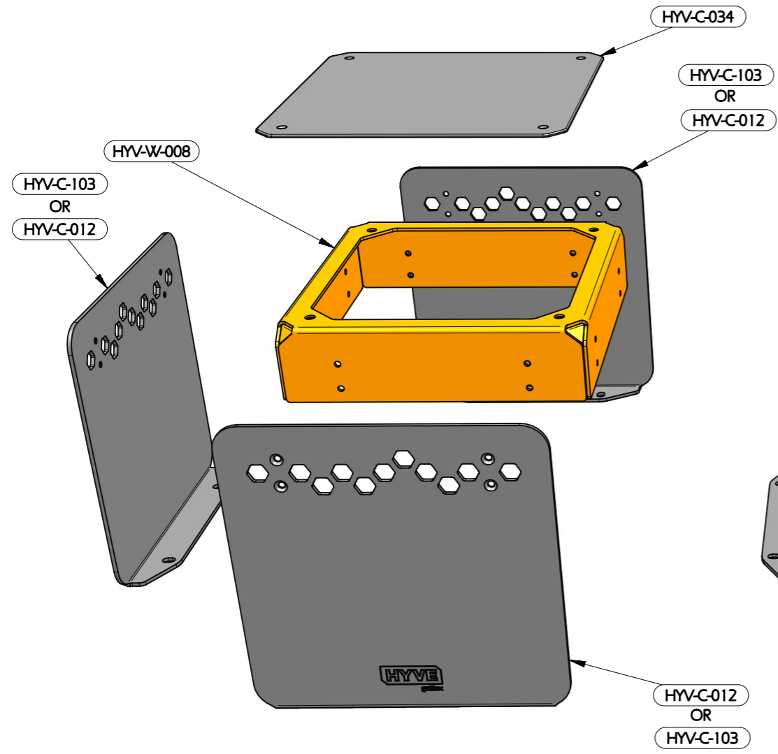
HYVE 90 DEGREE CONNECTOR
