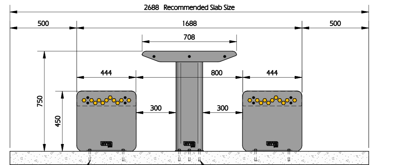
SIDE VIEW
