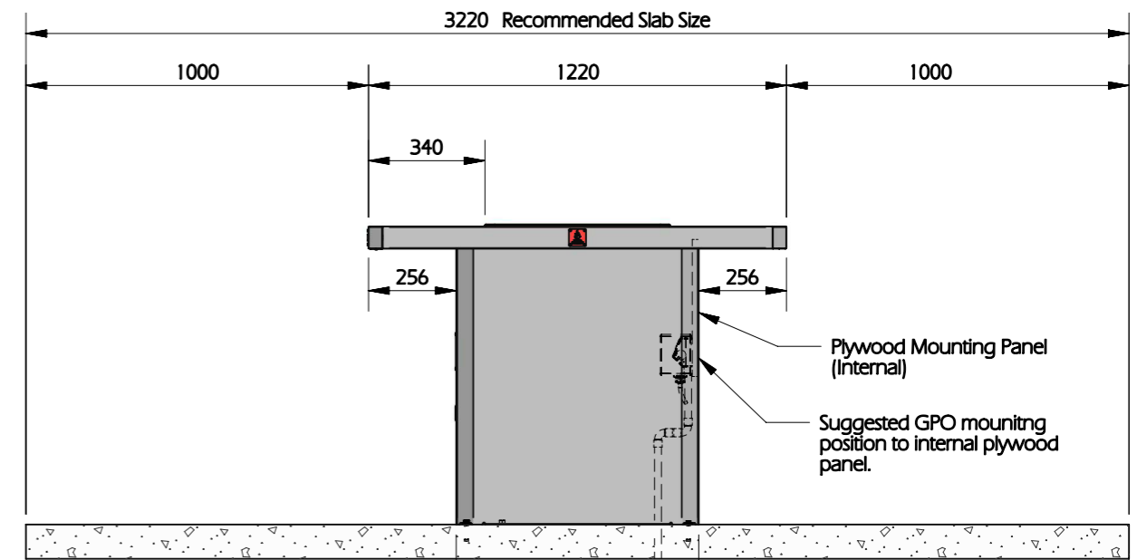
SIDE VIEW SCALE 1:20
