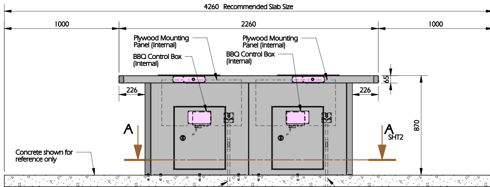
ELEVATION SCALE 1:20
