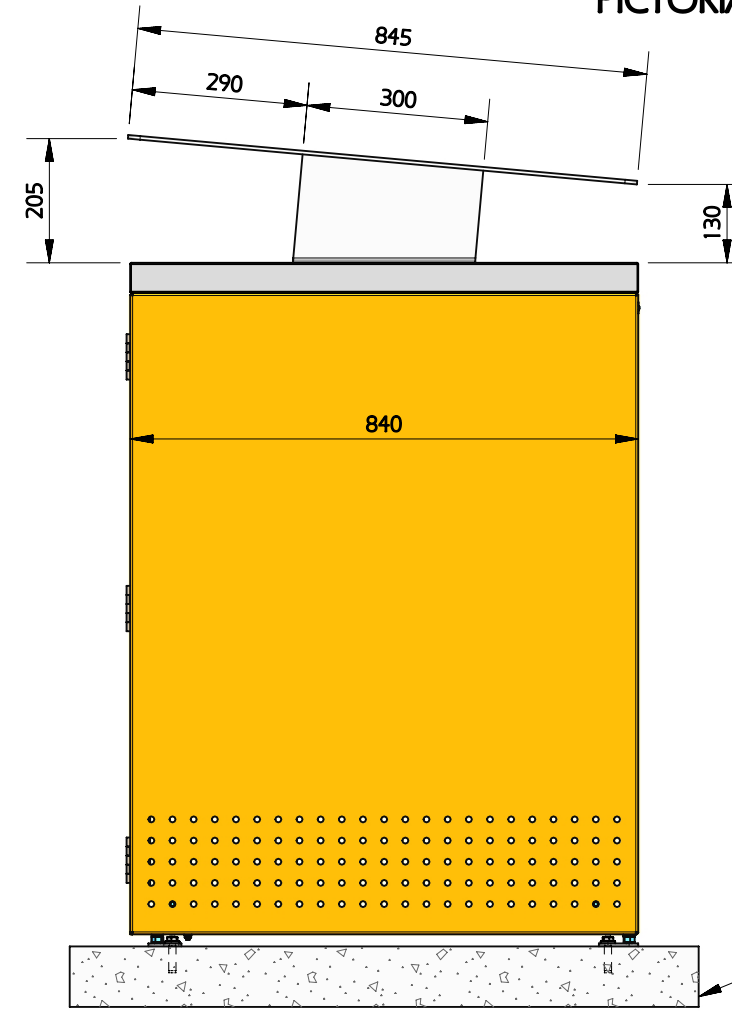
SIDE VIEW SCALE: NTS
