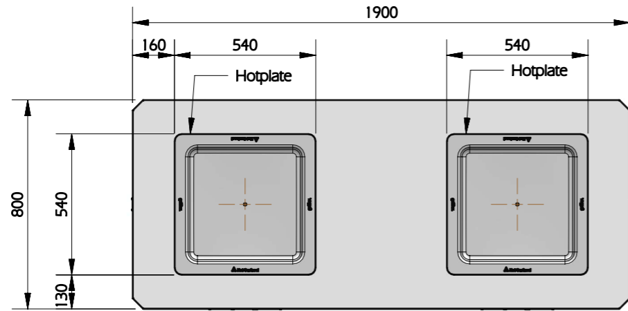
TOP VIEW SCALE 1:20
