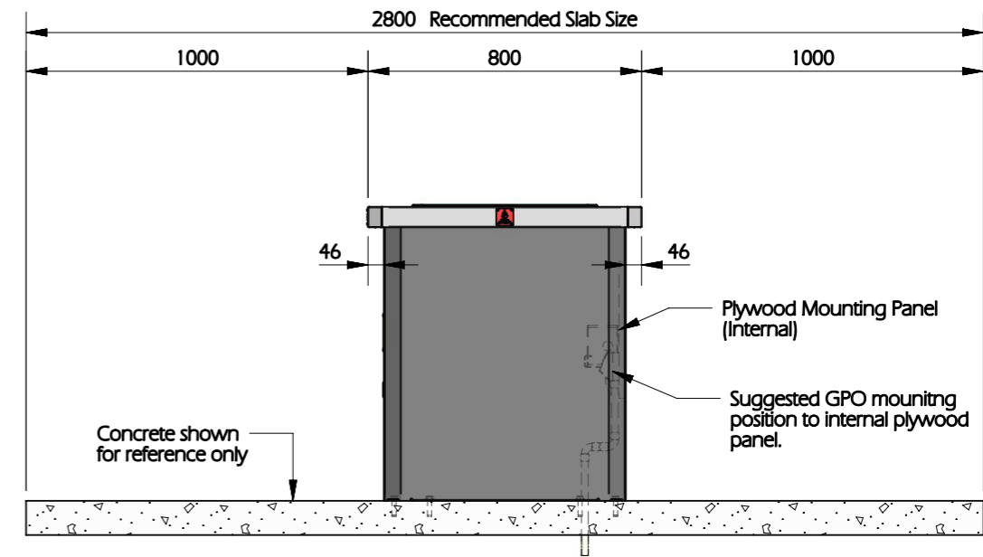
SIDE VIEW SCALE 1:20
