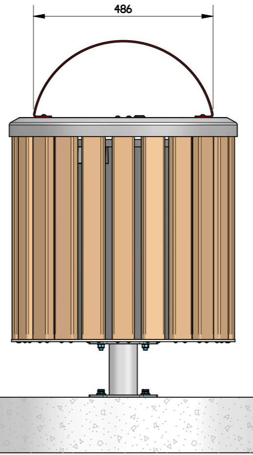
SIDE VIEW SCALE: NTS
