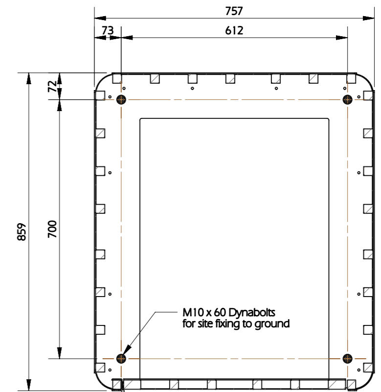
FOOTPRINT SECTION A-A SCALE 1:10
